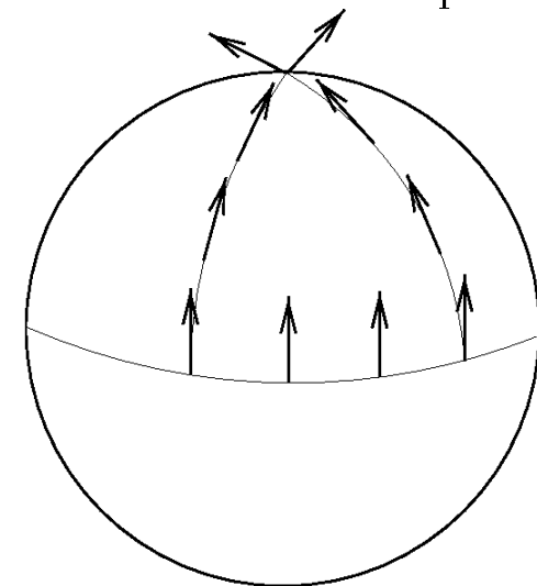
Example of parallel transport on 2-sphere
